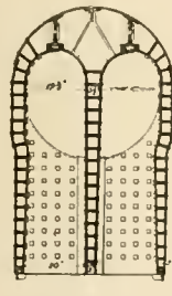
Section of Firebox FIG. 57.
